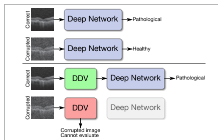
Fig. 2: Top: An automatic diagnosis method with no validation. However, the presence of corruption —noise in this case— leads to an erroneous healthy prediction. Bottom: Our DDV model learns the data distribution the network was trained on, and prevents any diagnosis when it detects an image outside the distribution.
