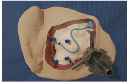
Fig. 3: A model of a patient-specific planning for robotic lead channel milling. The channel stores the excessive lead under the surface of the mastoid bone. The fiducial screws and the tripod are used for the image-guidance.
